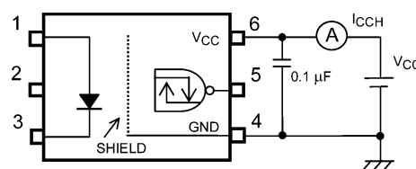
Fig. 13.1.4 ICCCH Test Circuit
