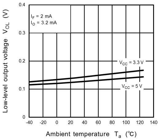
Fig. 13.2.4 V_{OL} - T_a
