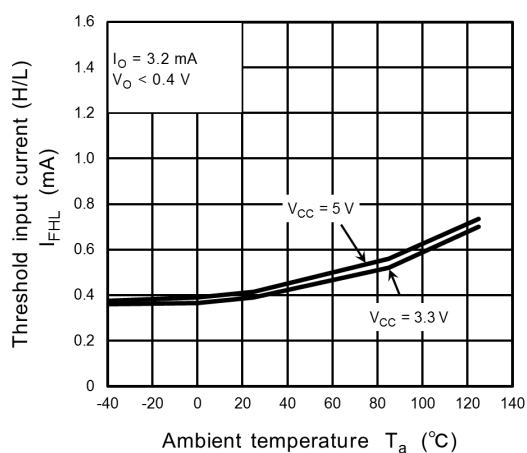
Fig. 13.2.9 I_{FHL} - T_a
