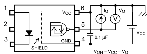
Fig. 13.1.2 VOH Test Circuit
