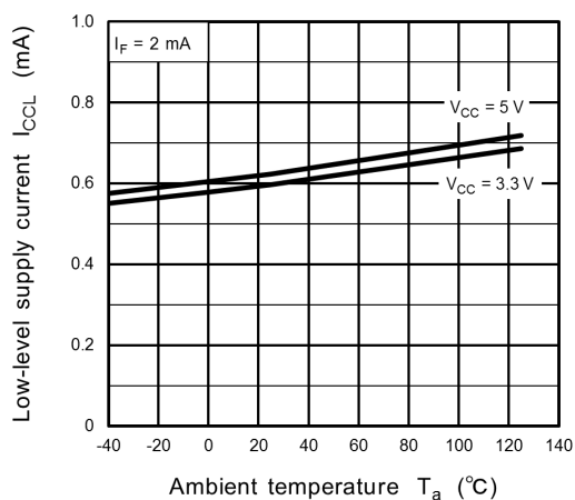
Fig. 13.2.7 I_{CCL} - T_a
